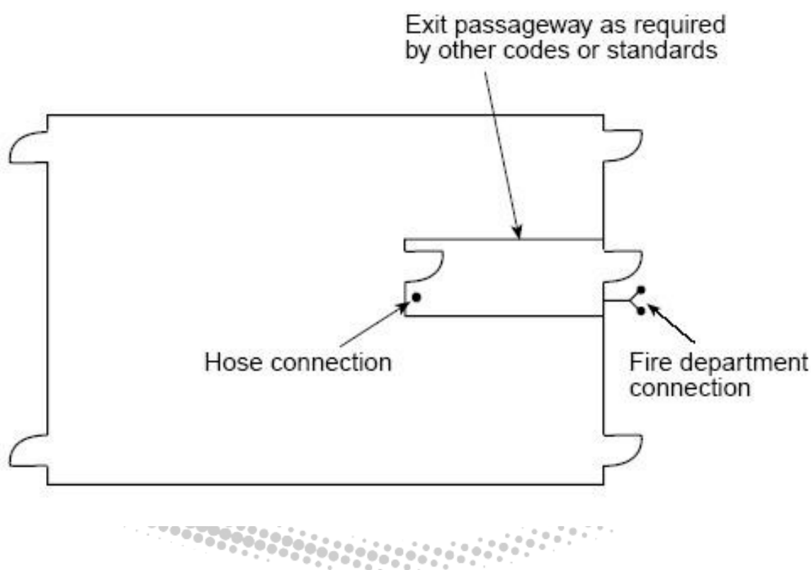
FIGURE A-5-3.2(c) Location of hose connections in exit passageways.
